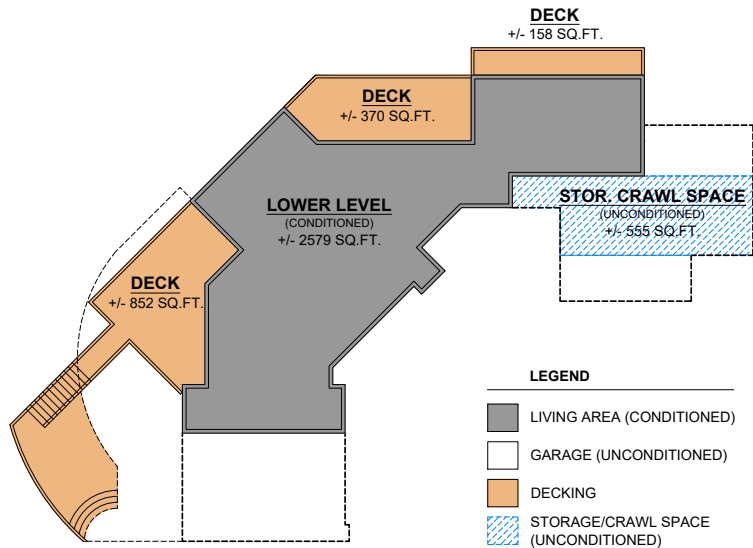
LOWER LEVEL SCALE: 3/32"=1'-0"
